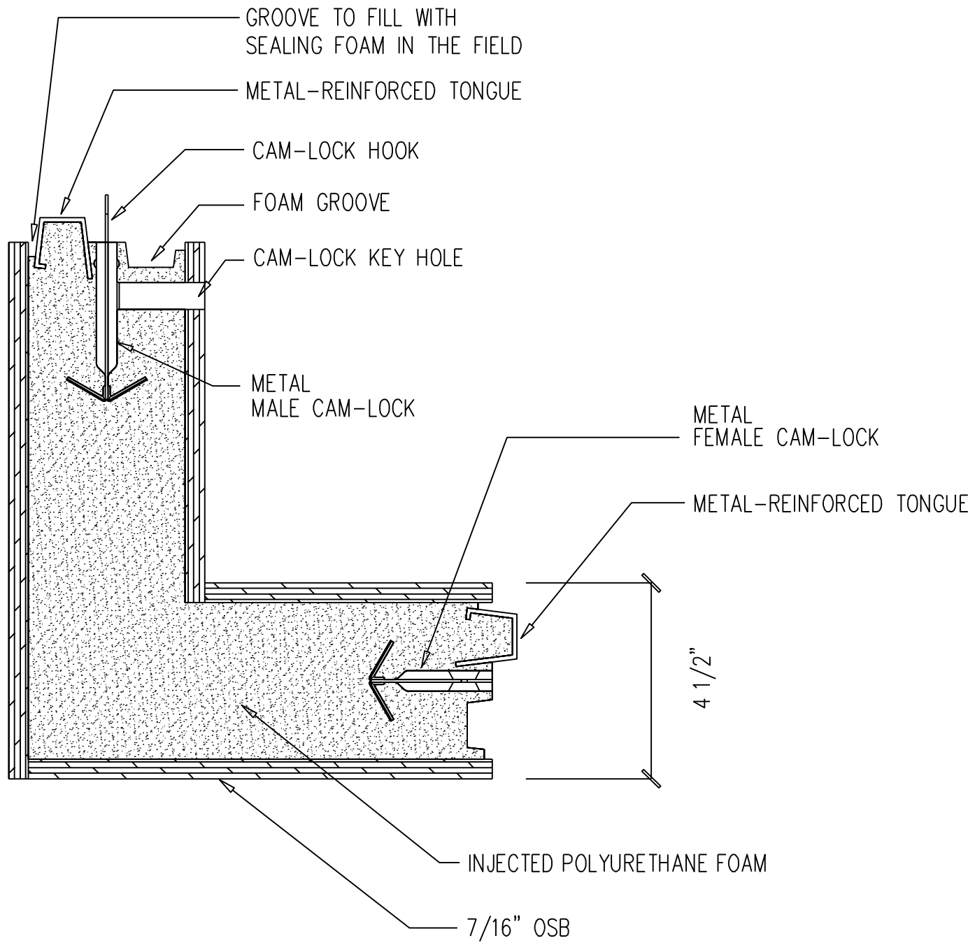
4.5" ICS ONE PIECE CORNER PANEL CROSS SECTION DETAIL
